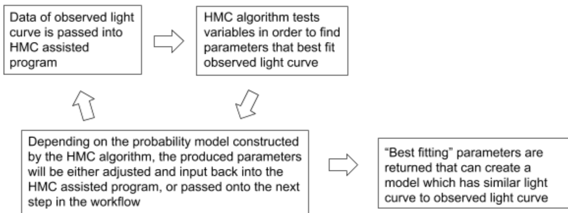
Figure 3: Workflow involved with using the HMC algorithm
